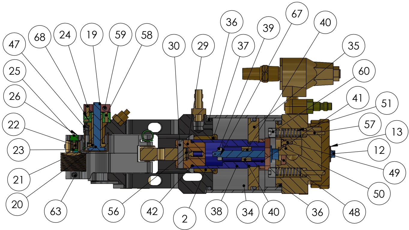
SECTION B-B
