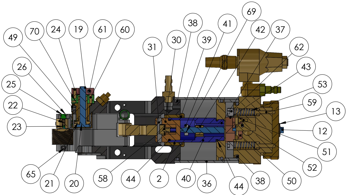
SECTION B-B
